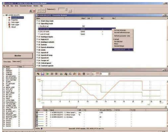
DriveStudio
