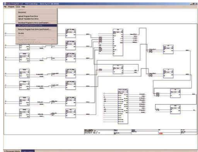
DriveSPC
